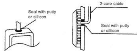
To lead wiring from top of remote sensor, To lead wiring from rear of remote sensor,
